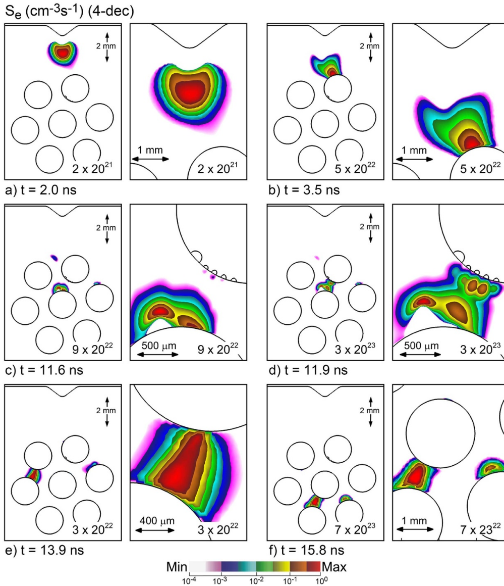
Figure 5. Time evolution of electron impact source in the full-size base-case reactor. (a) 2.0 ns, (b) 3.5 ns, (c) 11.6 ns, (d) 11.9 ns, (e) 13.9 ns and (f) 15.8 ns. At each time, images are shown for the (left) full reactor and (right) enlargements in regions of interests. Sources are plotted on a 4 decade log scale with the maximum value indicated in each frame.
