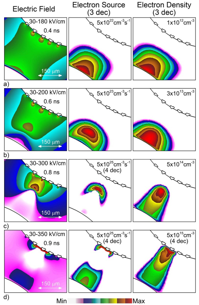
Figure 9. Plasma properties in the vicinity of protruding catalytic particles (left to right) electric field, electron impact ionization source and electron density at times of (a) 0.4 ns, (b) 0.6 ns, (c) 0.8 ns and (d) 0.9 ns. Electron density and source are plotted on a 3 decade log-scale unless indicated otherwise. The maximum value or range of values plotted in the image are indicated in the frame.
