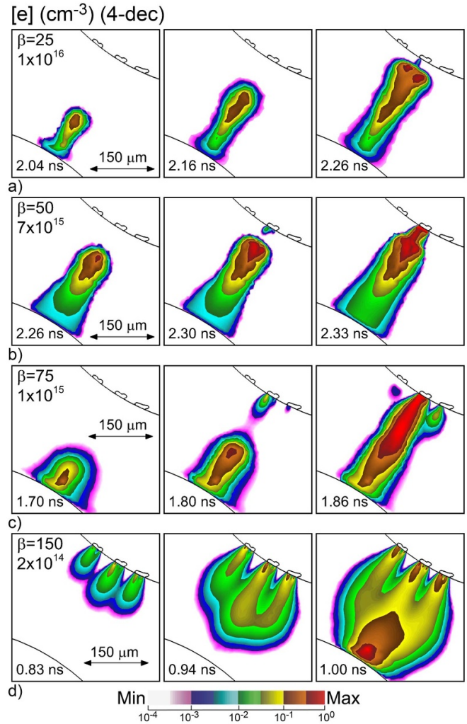
Figure 10. Electron densities at the end of the voltage pulse for different values of the electric field enhancement factor, \beta , in the reduced geometry at different times (left to right). \beta = (a) 25, (b) 50, (c) 75 and (d) 150. Densities are plotted on a 4 decade log-scale with maximum values noted in each frame. The mechanism of plasma formation changes from being volume to surface dominated with increasing \beta .
