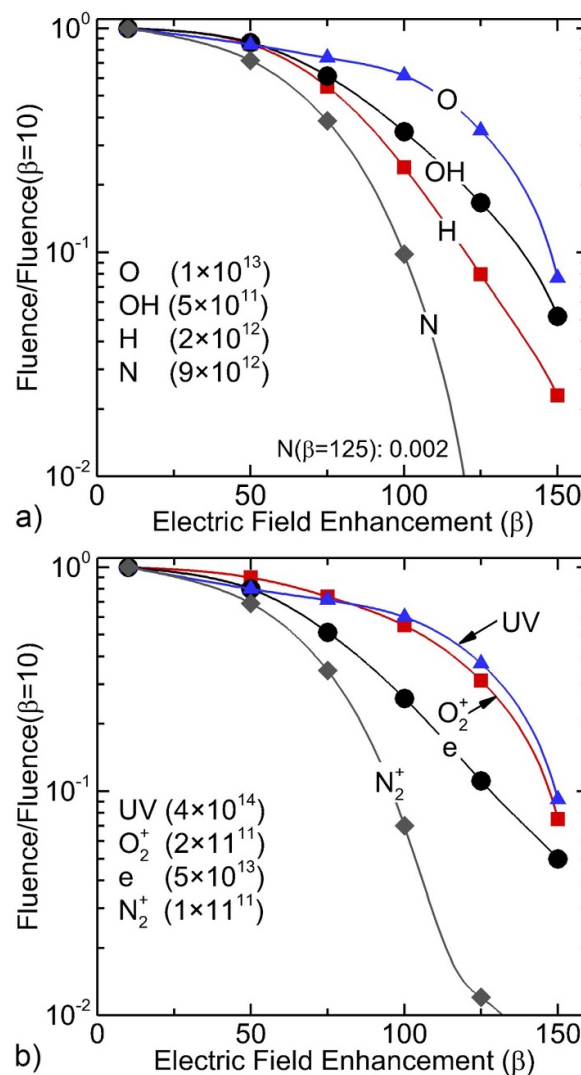
Figure 12. Fluences of selected species to the surfaces of the middle catalyst particle as a function of electric field enhancement factor for the reduced-scale geometry. (a) O, OH, H, N and (b) N_2^+ , O_2^+ , UV photons and electrons. Values are normalized by the fluence for \beta=10 . With the increase in conductivity due to electric field emission of electrons, the electric field in the adjacent plasma decreases, leading to a colder plasma and decreased fluences to the surface.
