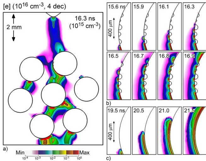
Figure 7. Electron density in the full-size geometry with catalysts arranged along the left equator of the topmost particle. (a). Electron density in entire reactor at 16.3 ns. (b) Surface ionization wave (SIW) in the vicinity of the catalysts (15.6 ns–16.9 ns) showing stagnation of SIWs approaching the catalysts and re-ignition on the other side. (c) SIW for the same location without metallic catalysts. Densities are plotted on a 4 decade log scale.
