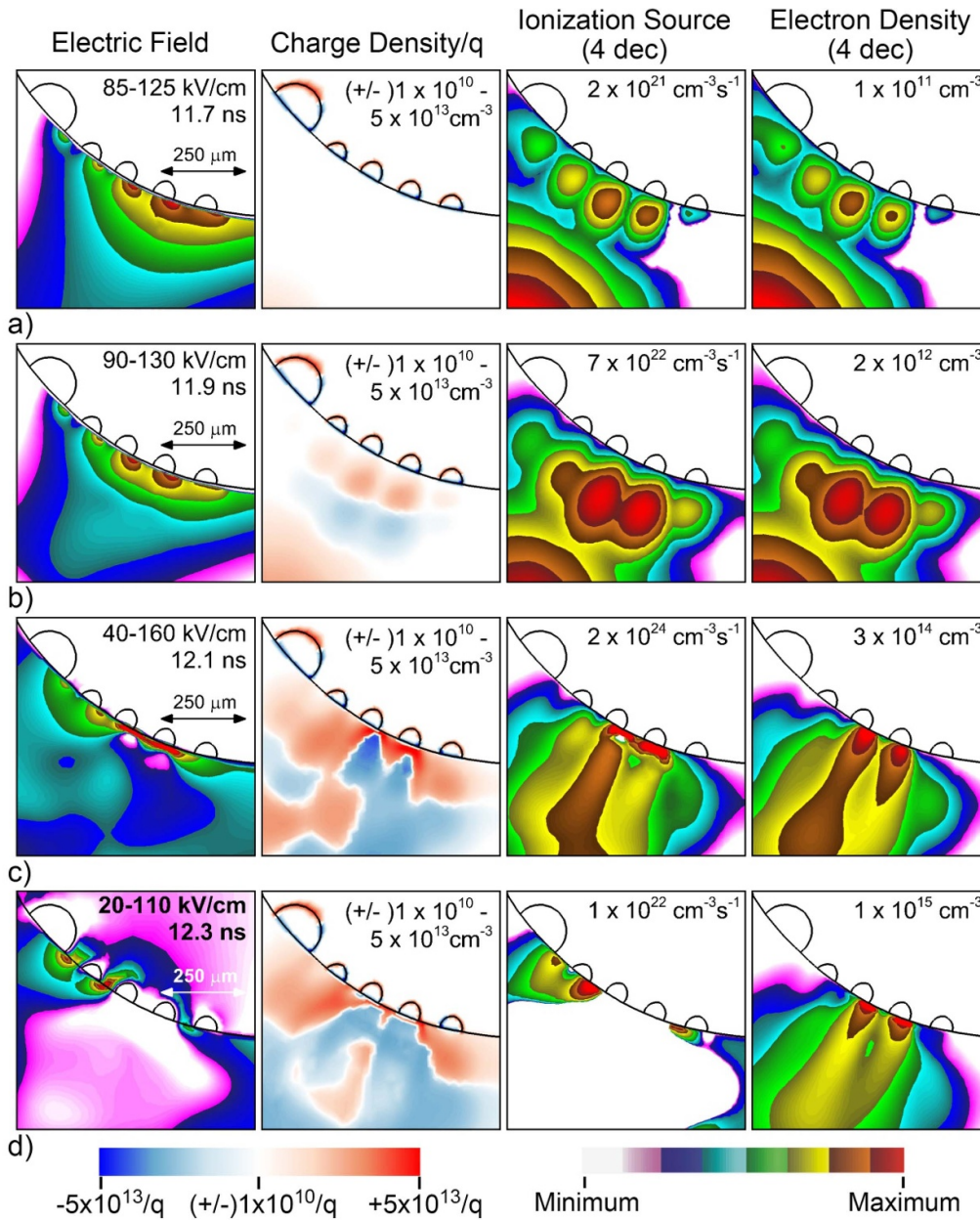
Figure 6. Plasma properties in the vicinity of the catalyst particles (left to right) electric field, charge density, ionization source term and electron density at times of (a) 11.7 ns, (b) 11.9 ns, (c) 12.1 ns and (d) 12.3 ns. These images are during streamer propagation toward the metallic catalysts. Gradients in charge density lead to formation of strong electric fields, and electric field emission of electrons from the surfaces of metals.
