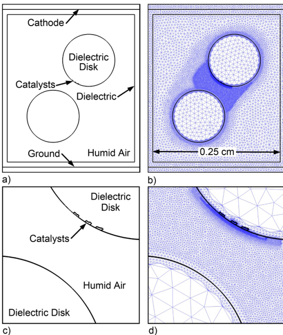
Figure 2. Geometry of the reduced scale reactor. (a) Schematic of the entire reactor, (b) computational mesh, (c) enlargement of inter-disk gap and catalysts and (d) enlargement of numerical mesh.
