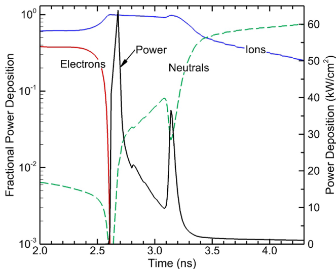
Figure 13. Total and fractional power deposition to the surface of catalyst as a function of time for the reduced scale geometry base case. Power deposition by ions dominates during the discharge pulse, with neutral chemical reactions dominating in the afterglow.
