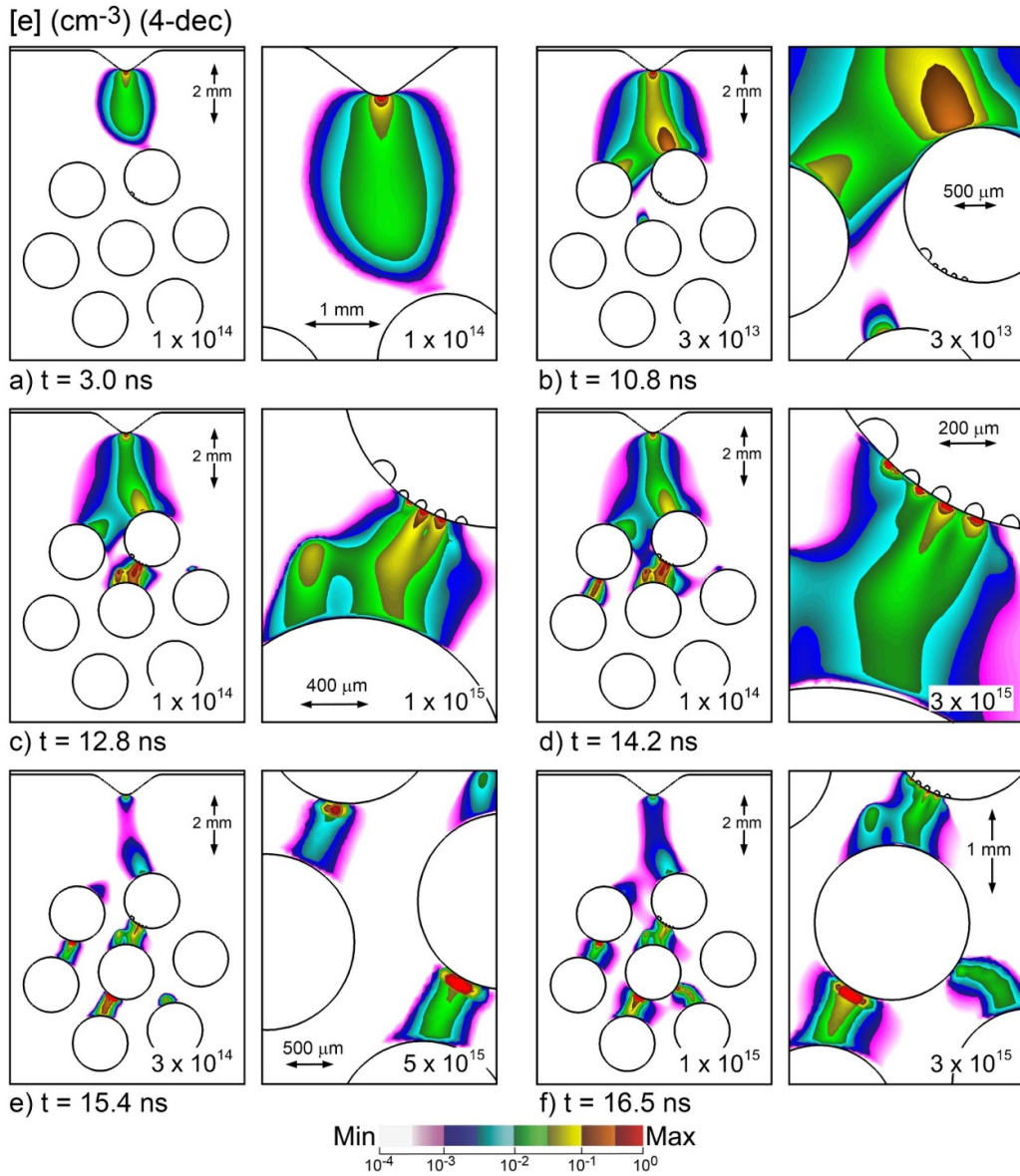
Figure 4. Time evolution of electron density in the full-size base-case reactor. (a) 3.0 ns, (b) 10.8 ns, (c) 12.8 ns, (d) 14.2 ns, (e) 15.4 ns and (f) 16.5 ns. At each time, images are shown for the (left) full reactor and (right) enlargements in regions of interests. Densities are plotted on a 4 decade log scale with the maximum value indicated in each frame.
