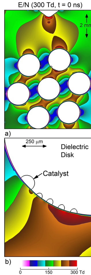
Figure 3. Reduced electric field ( E/N ) at t = 0 \text{ s} for (a) the full-size base-case geometry and (b) enlargement near the catalysts.
