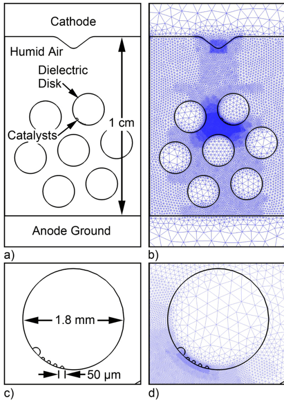
Figure 1. Geometry of the base case reactor. (a) Schematic of the entire reactor, (b) computational mesh, (c) enlargement of the topmost disk and (d) enlargement of numerical mesh.
